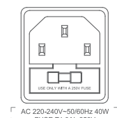
AC 220-240V~50/60Hz 40W FUSE T1.6AL 250V
